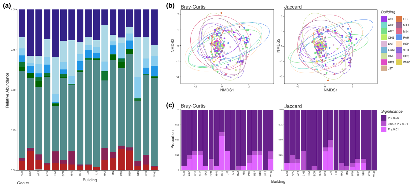
FIGURE 2 Composition of mycobial communities by building. (a) Fungal composition: Relative abundances of top genera (>1%) by building shown. Family of genera is italicized and in brackets below genus in the legend. (b) Beta diversity. Non-metric multidimensional scaling (NMDS) plots of dissimilarity metrics. Each point represents a sample; color indicates building. (left) Bray-Curtis (abundance) and (right) Jaccard (presence-absence). (c) Post-hoc Tukey analysis: Percentage on y-axis of non-significant ( p > 0.05 ), significant ( 0.05 \geq p > 0.01 ), and highly significant ( p \leq 0.01 ), as indicated by color, building interactions. Henley business school (HBS) had the highest percentage of significant values (50% or more) therefore, its composition significantly differed from half or more of the buildings. Building abbreviations as follows; AGR, Agriculture; ARC, Archaeology; ART, Art; CHE, Chemistry; EAT, Eat at the Square; EDM, Edith Morely; HNU, Harry Nunsten; HBS, Henley Business School; JJT, JJ Thompson; LIB, Library; MAT, Maths; MINL, Mingella; PAH, Park House; RSP, Sports Park; STU, Student Union; URS, URS; WHK, Whiteknights.
