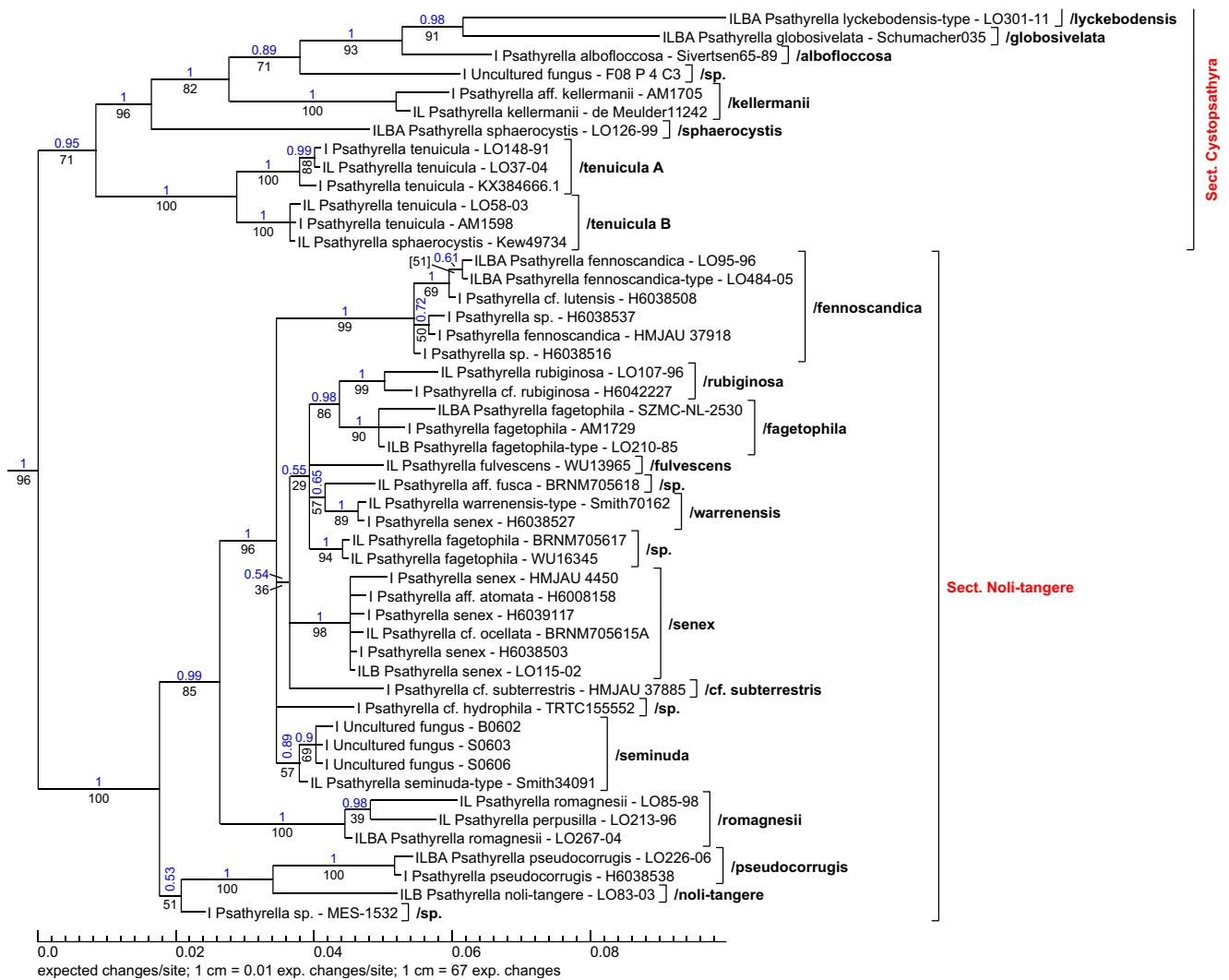
Fig. 69 Phylogram part of the sections Cystopsathyra and Noli-tangere ; position in tree see Fig. 67
