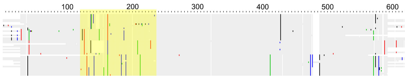
Fig. 95 ITS alignment of the “lagopus A” down to “pachyderma” clade. Coloured sites (in AliView colour code) represent the difference from majority rule consensus. Grey areas are sites which match the
