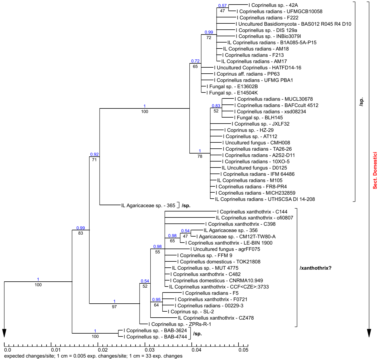
Fig. 53 Phylogram part of the section Domestici ; position in tree see Fig. 47
