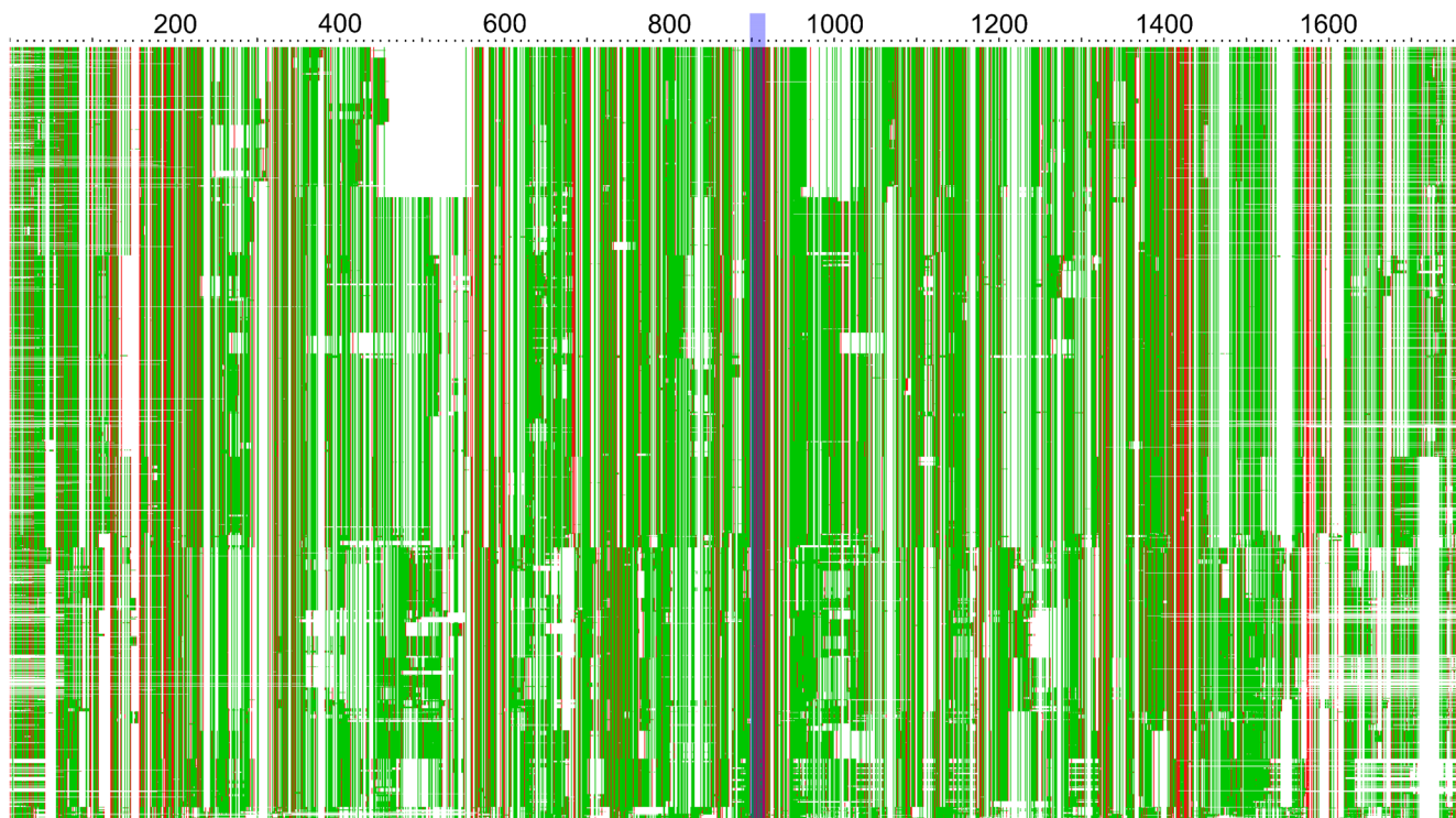
Fig. 27 Sequential gap matrices of the ITS1, 5.8S and ITS2 regions after the last iteration step. Green stands for gap not present; red stands for gap present; white: no indel data in this region; blue background: 5.8S gap matrix; representation from AliView; the scale represents the site numbering
