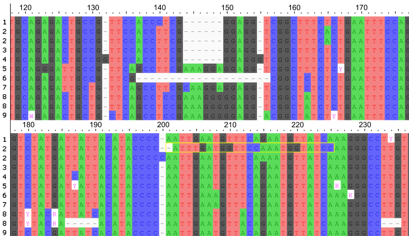
Fig. 96 Genetic key to separate the nine clades: 1 = C. lagopus A; 2 = C. lagopus B (note the 2 different rows); 3 = C. lagopus C; 4 = C. lagopus D; 5 = C. lagopus E; 6 = C. lagopus F; 7 = C. lagopus G; 8 = C. brunneofibrillosa ; 9 = C. pachyderma . The yellow framed area is
