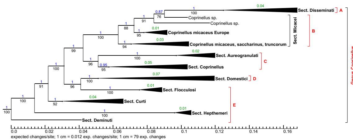
Fig. 47 Partial view from the total phylogram of the genus Coprinellus , collapsed to section level; position in tree see Fig. 42. Red brackets are references to detailed phylograms: A = Fig. 48; B = Fig. 49; C = Fig. 52; D = Fig. 53; E = Fig. 54
