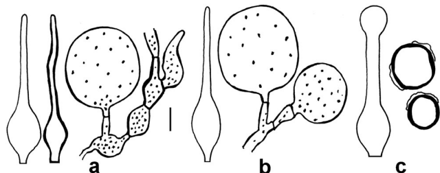
Fig. 60 a–c Pileocystidia and veil elements of some members of the genus Coprinellus . a C. hepthemerus , AM1181; b C. dilectus , AM1749; c C. curtus , 18.IX.2006, A. Melzer, no voucher; scale bar 10 \mu m; Drawing: A. Melzer
